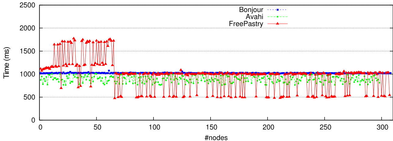
Fig. 10. Elapsed times for sequential registrations of services for Bonjour, Avahi and Free-Pastry
